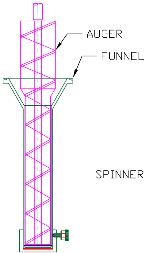
SELF FEED TOOLING
